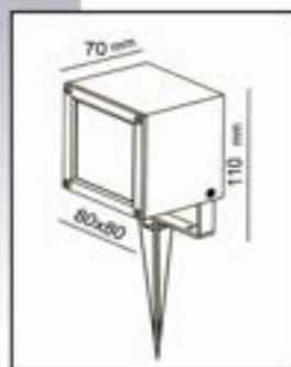
93 2741LEDSPIKE black 4x2W 460lm 3000K IP54 (incl. spike and 3m cable)
