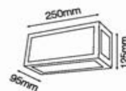
E3200B black LED 6W 310lm 3000K IP54
