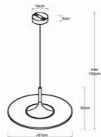
Bow black 230V 45W 4540lm 3000K dimmable 93 21
